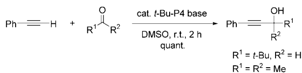
Scheme 2. 1,2-Addition of phenylacetylene to carbonyl compounds.
